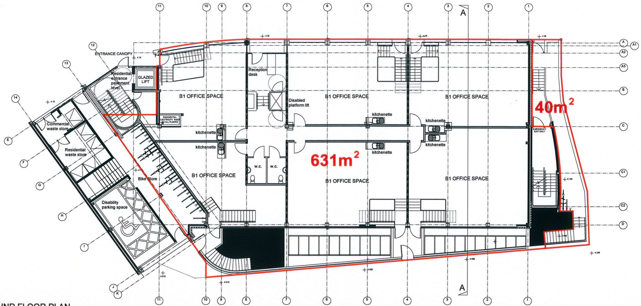
GROUND FLOOR PLAN LOWER GROUND FLOOR & GROUND FLOOR PLANS
